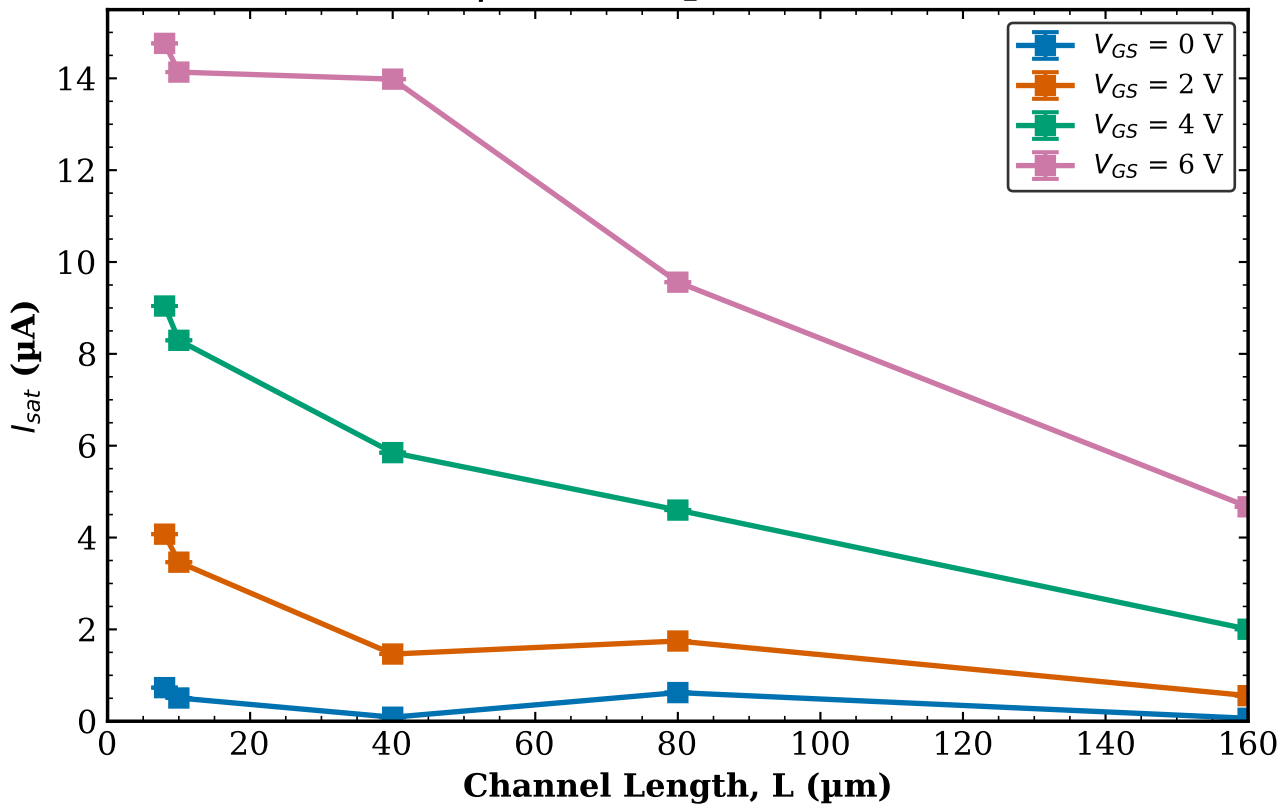
TFT1 Transistor 1 I_{sat} vs L | W = 50 \mu\text{m} (mean \pm std)
